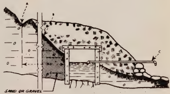
Fig. 33. PROPERLY PROTECTED SPRING (I)
